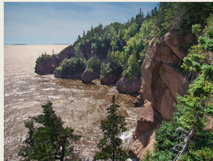
Obr. 6 Hopewell Rocks, záliv Fundy, NB
